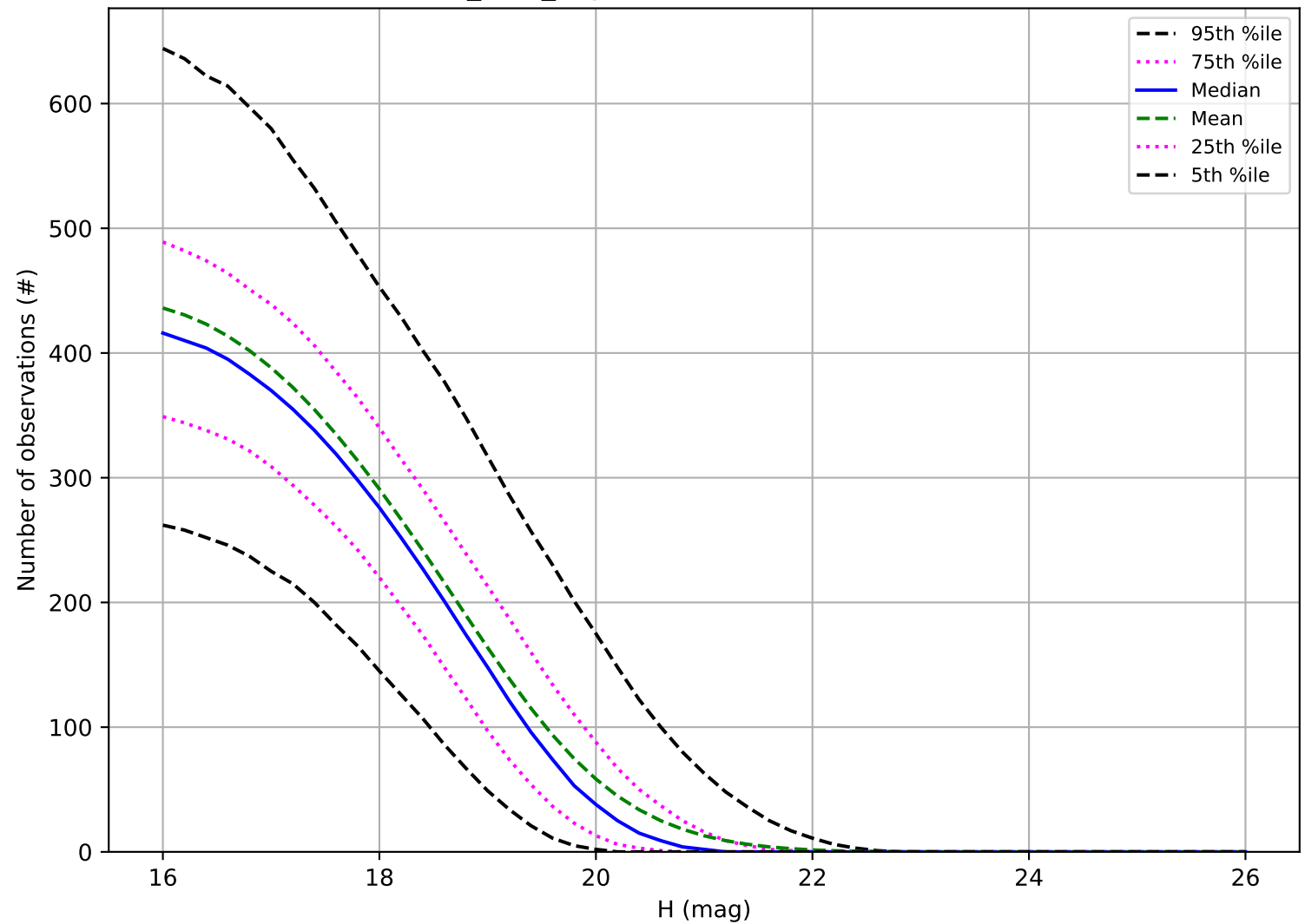
baseline_v3.0_10yrs: Number of observations MBA
