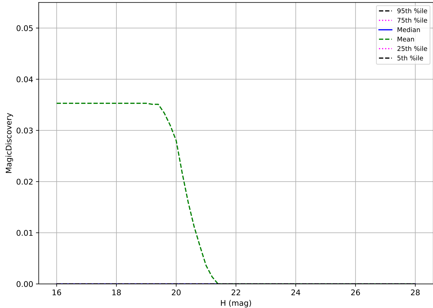
baseline_v3.0_10yrs: Vatira 6 detections in 60 nights detection loss
