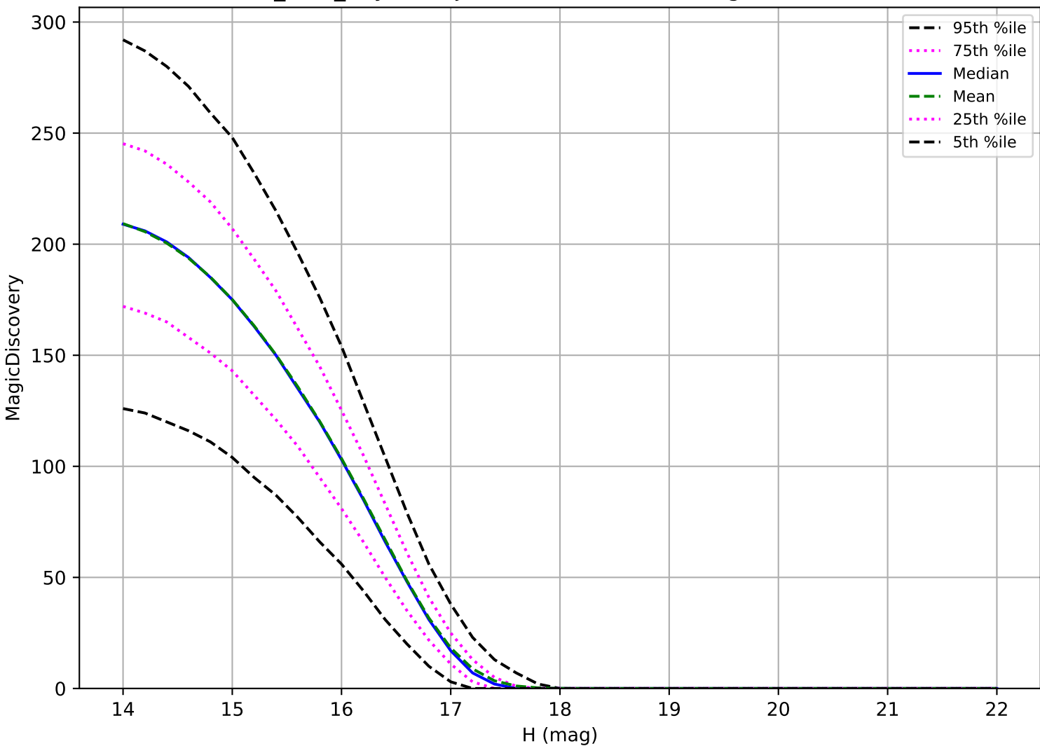
baseline_v3.0_10yrs: Trojan 6 detections in 60 nights detection loss
