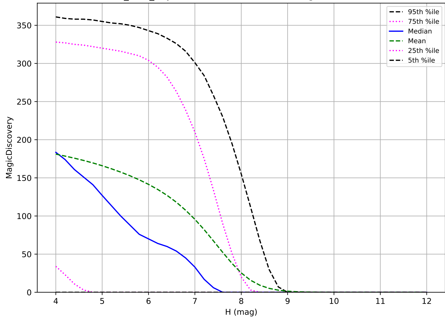
baseline_v3.0_10yrs: TNO 6 detections in 60 nights detection loss
