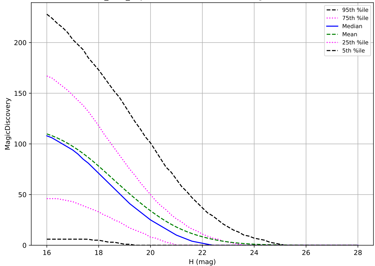
baseline_v3.0_10yrs: PHA 6 detections in 60 nights detection loss
