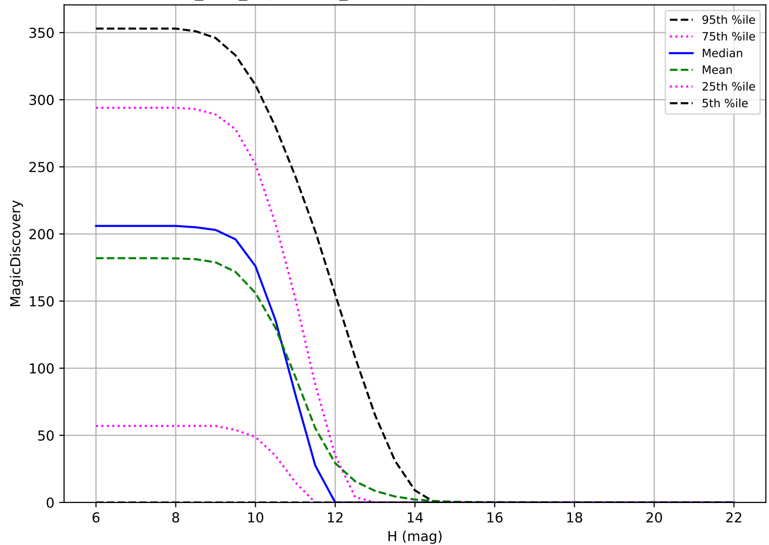
baseline_v3.0_10yrs: OCC_r20 6 detections in 60 nights detection loss
