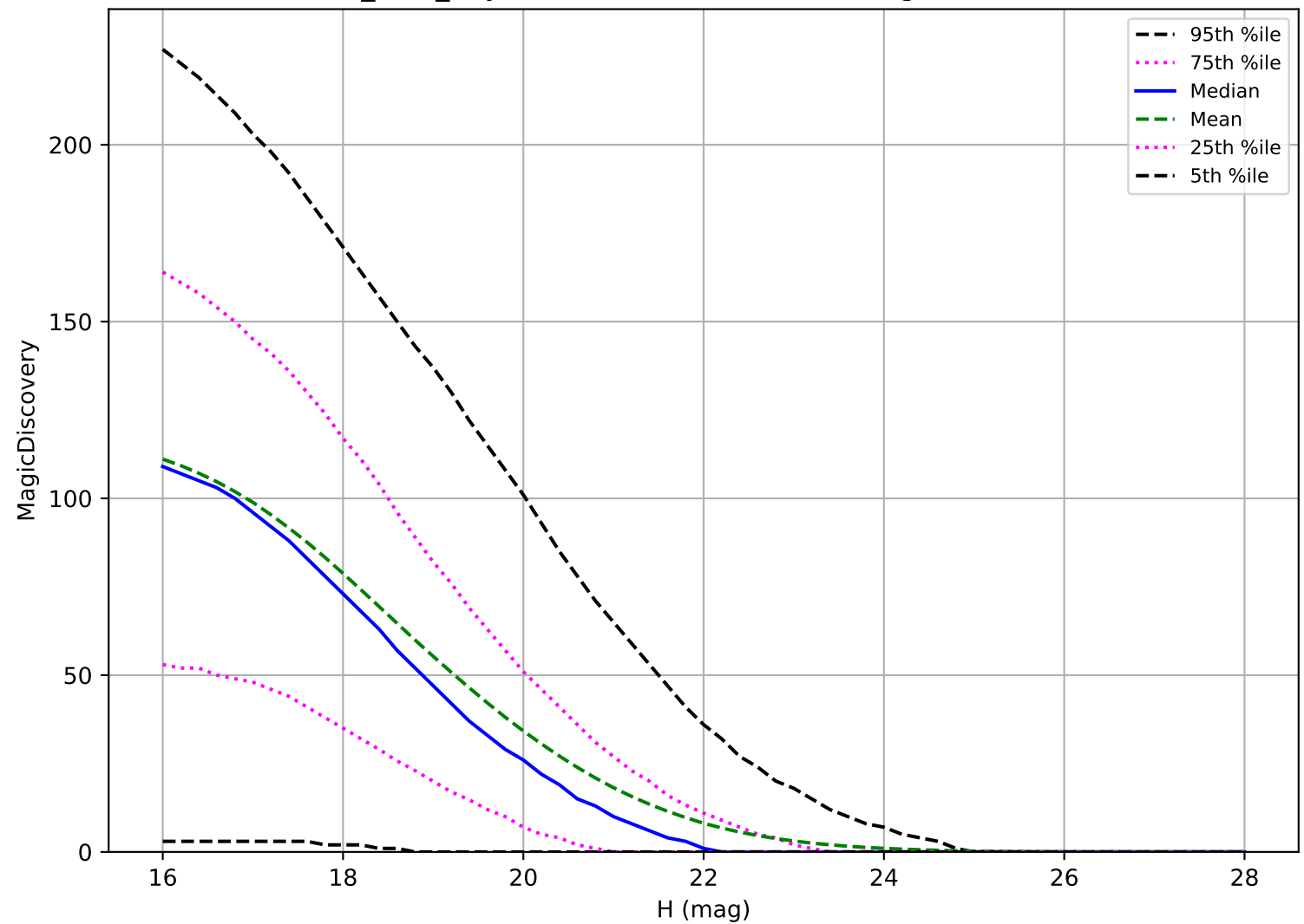
baseline_v3.0_10yrs: NEO 6 detections in 60 nights detection loss
