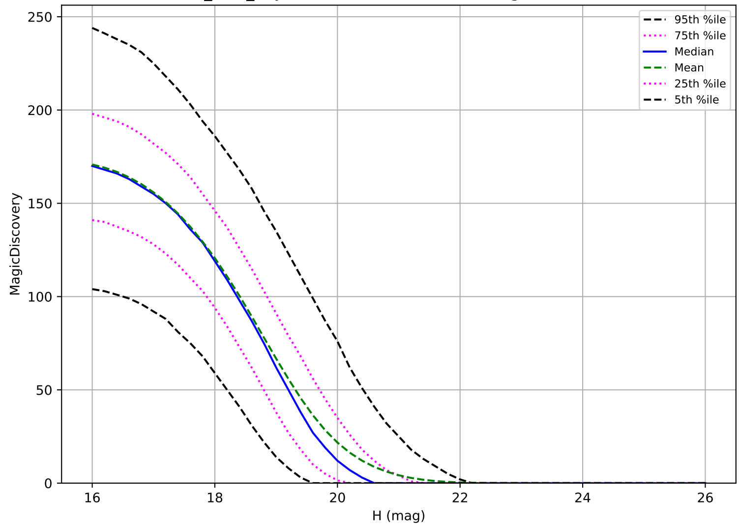
baseline_v3.0_10yrs: MBA 6 detections in 60 nights detection loss
