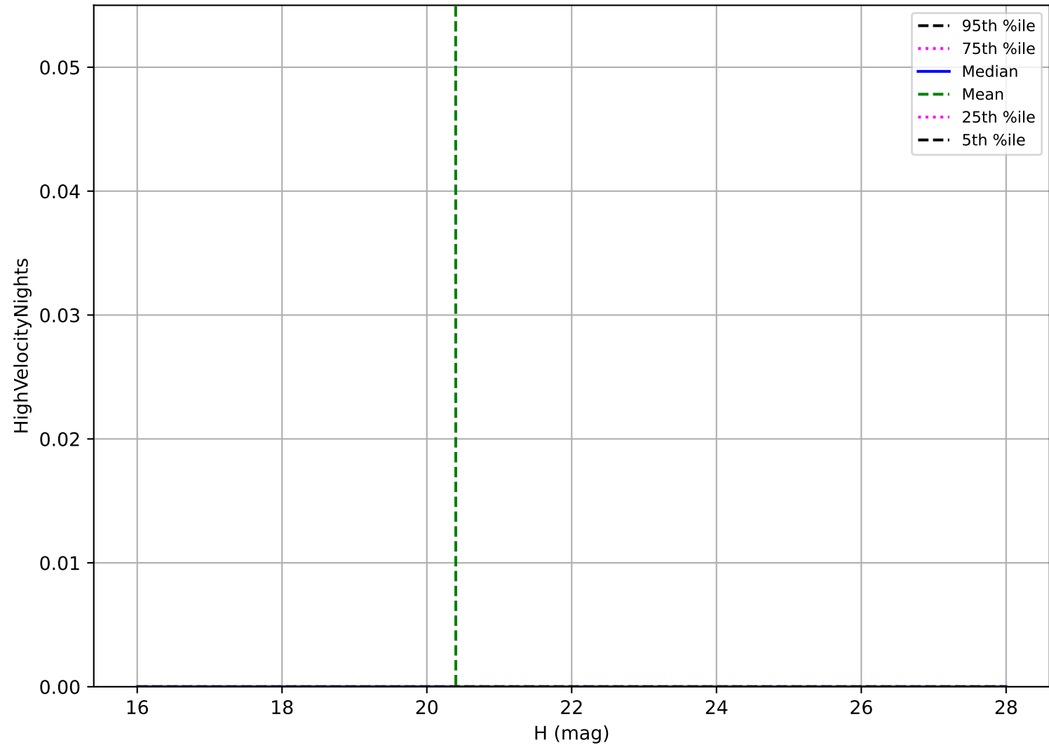
baseline_v3.0_10yrs: Vatira High velocity pair detection loss
