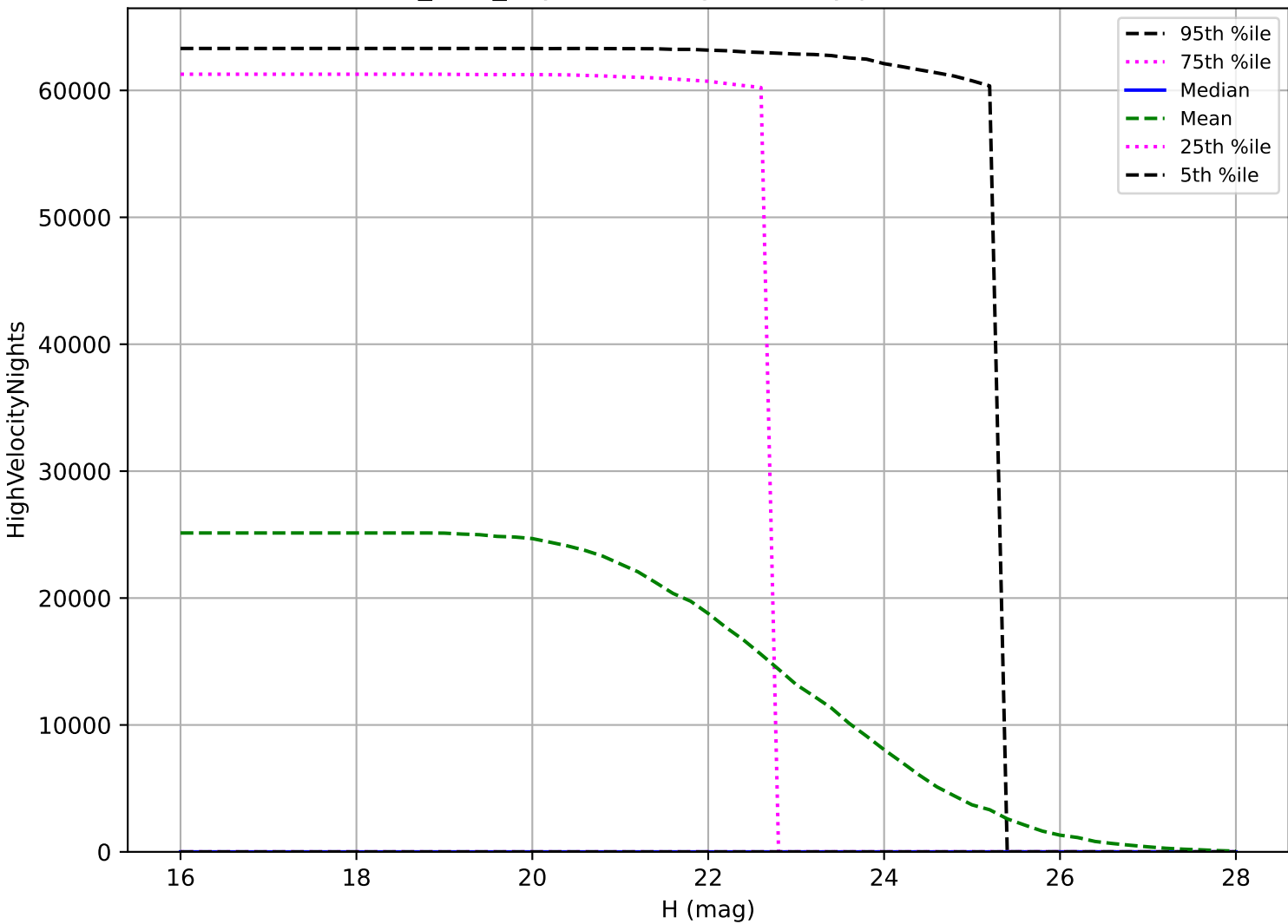
baseline_v3.0_10yrs: PHA High velocity pair detection loss
