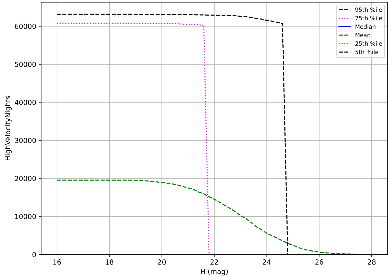
baseline_v3.0_10yrs: NEO High velocity pair detection loss
