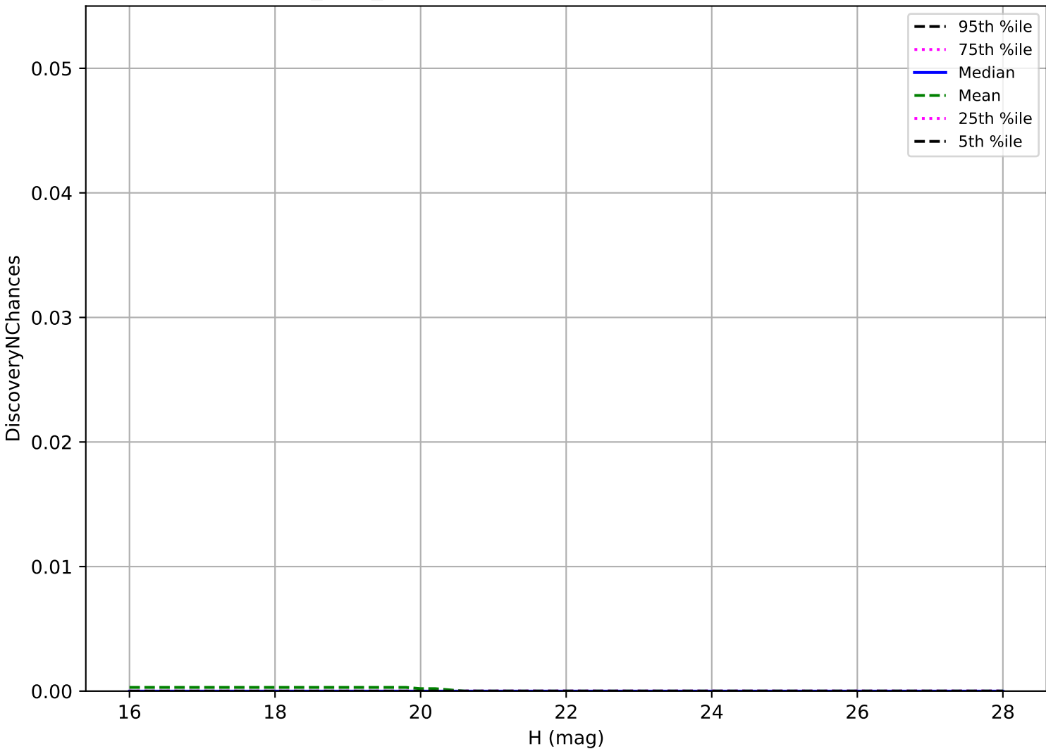
baseline_v3.0_10yrs: Vatira 3 pairs in 15 nights detection loss
