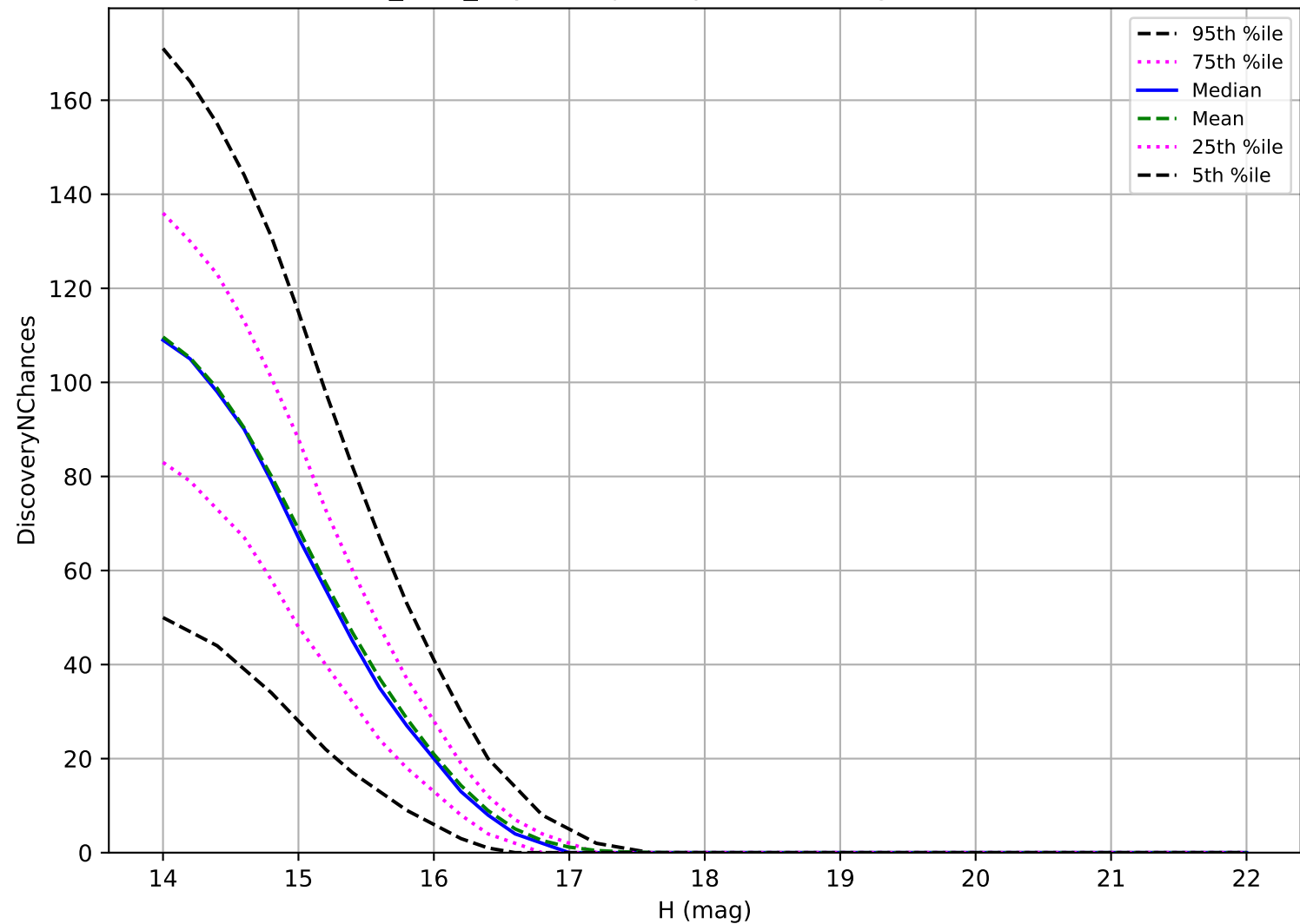
baseline_v3.0_10yrs: Trojan 3 pairs in 15 nights detection loss
