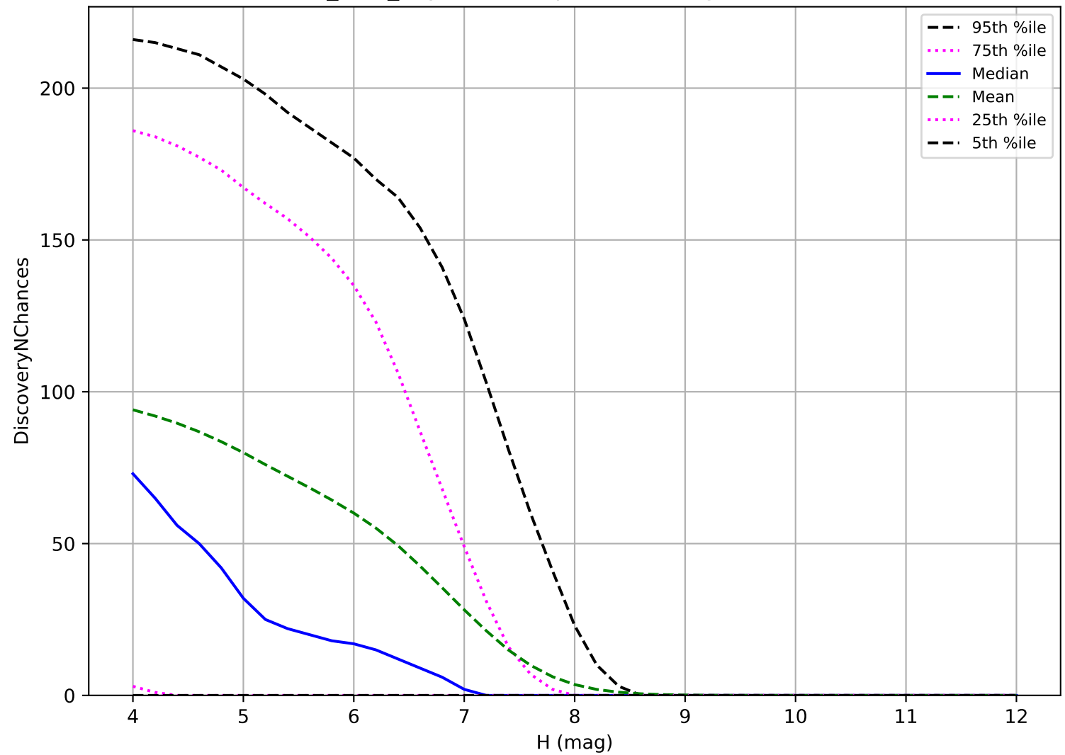
baseline_v3.0_10yrs: TNO 3 pairs in 15 nights detection loss
