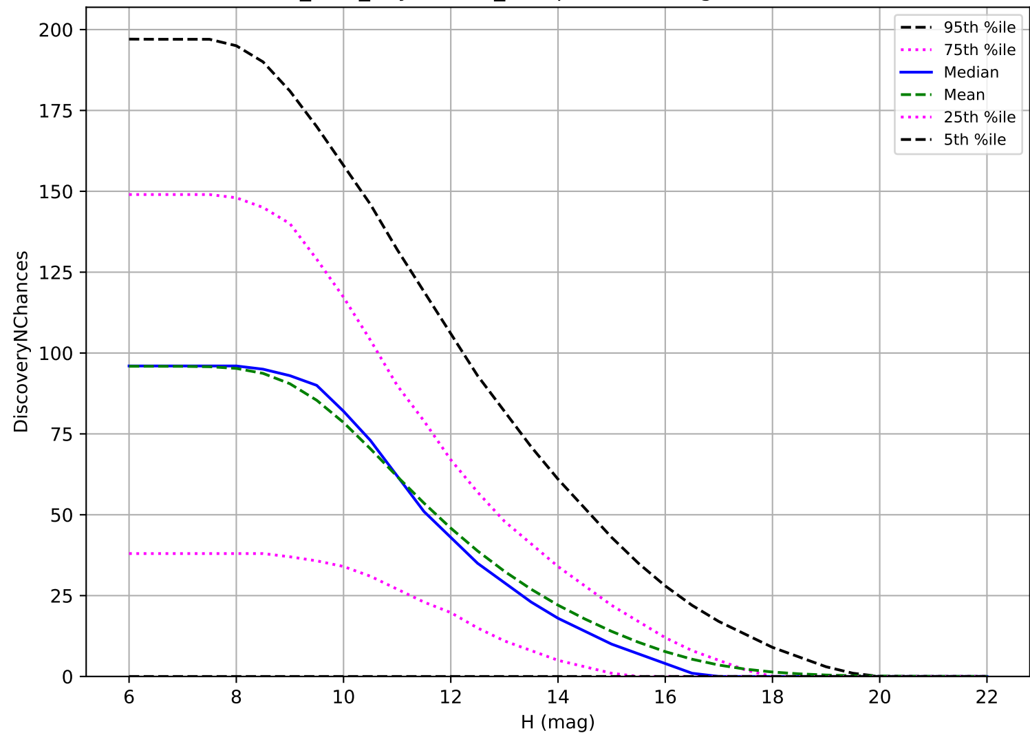
baseline_v3.0_10yrs: OCC_r5 3 pairs in 15 nights detection loss
