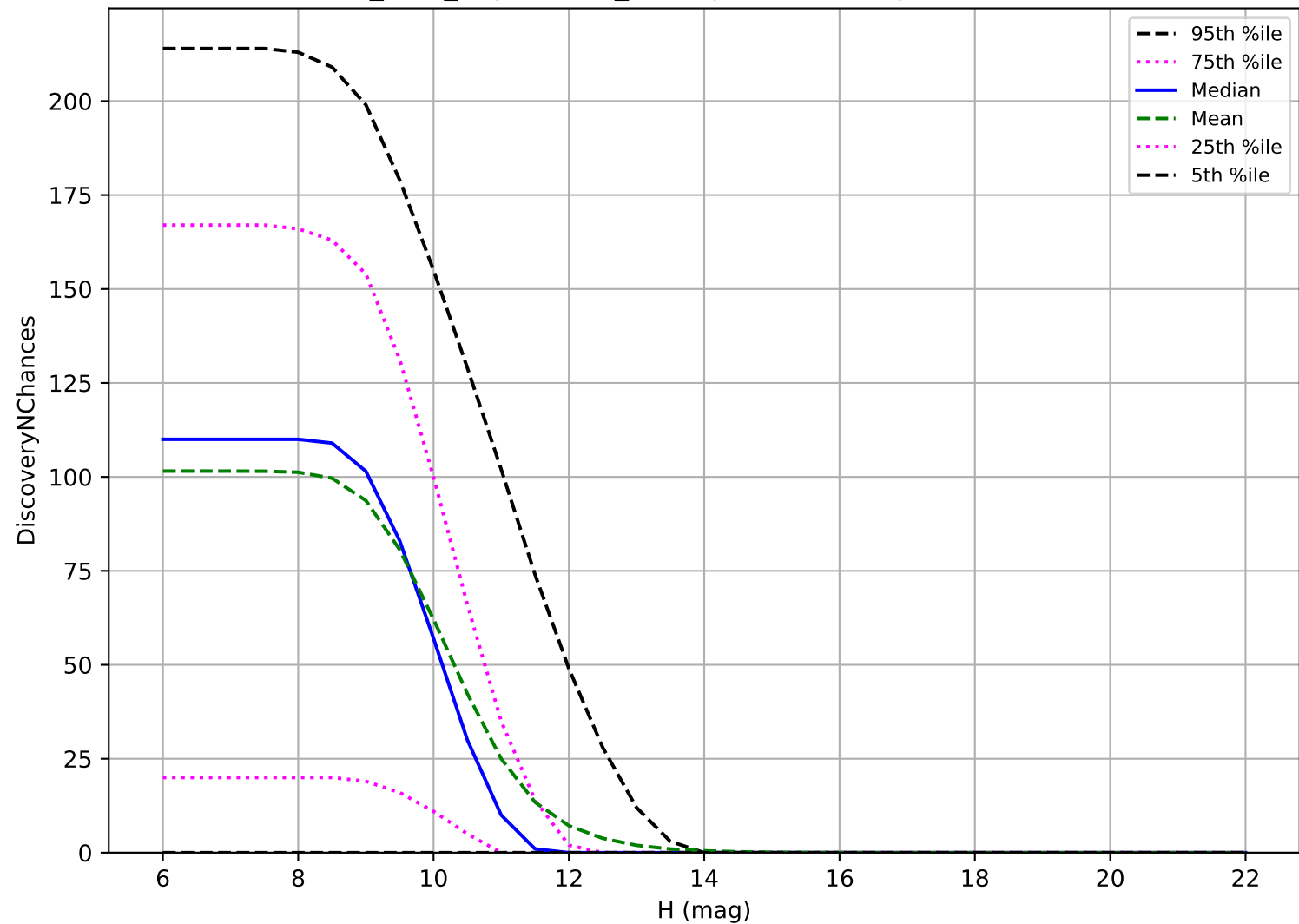
baseline_v3.0_10yrs: OCC_r20 3 pairs in 15 nights detection loss
