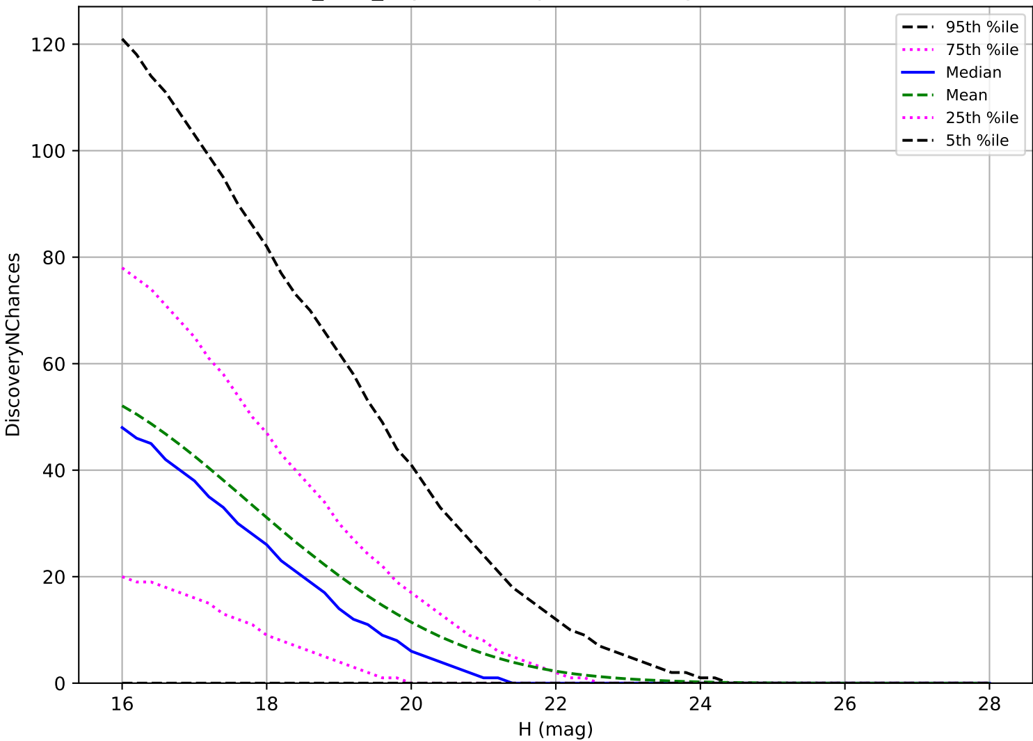
baseline_v3.0_10yrs: NEO 3 pairs in 15 nights detection loss
