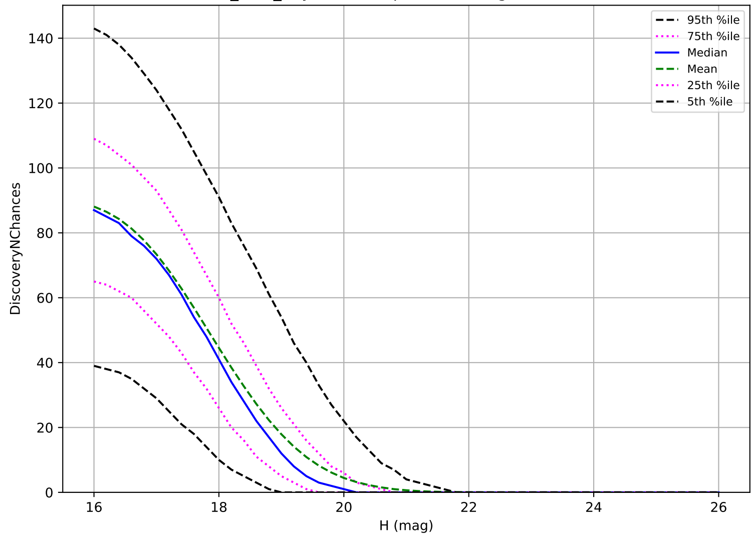
baseline_v3.0_10yrs: MBA 3 pairs in 15 nights detection loss
