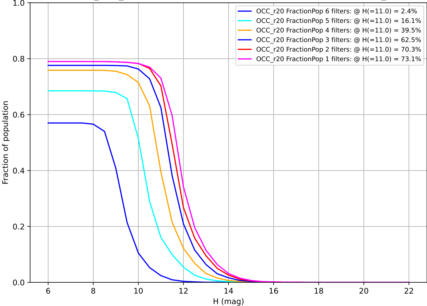
baseline_v3.0_10yrs: Fraction of population with colors in X filters OCC_r20
