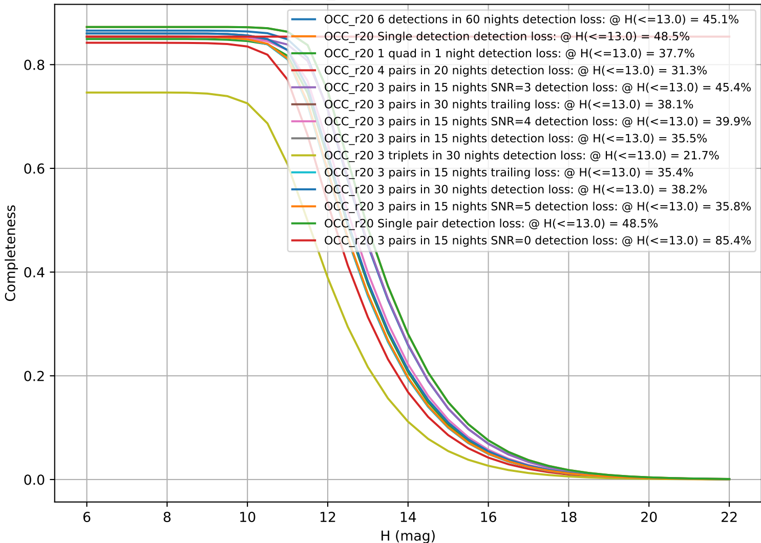
baseline_v3.0_10yrs: CumulativeCompleteness
