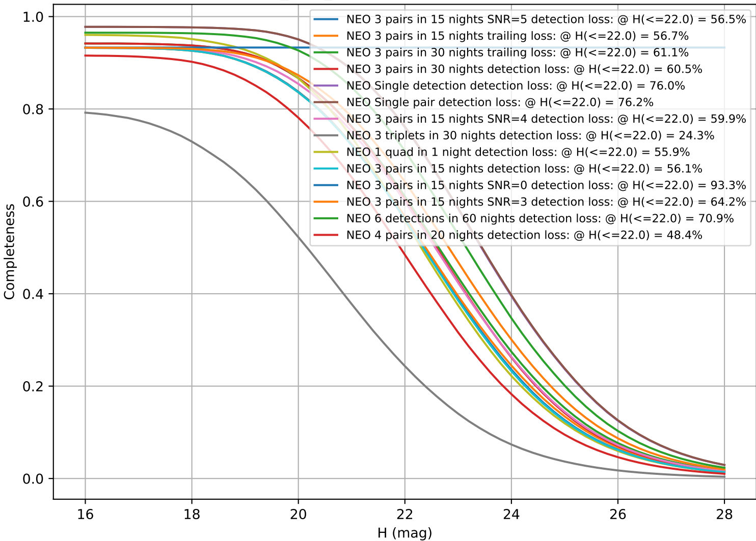
baseline_v3.0_10yrs: CumulativeCompleteness
