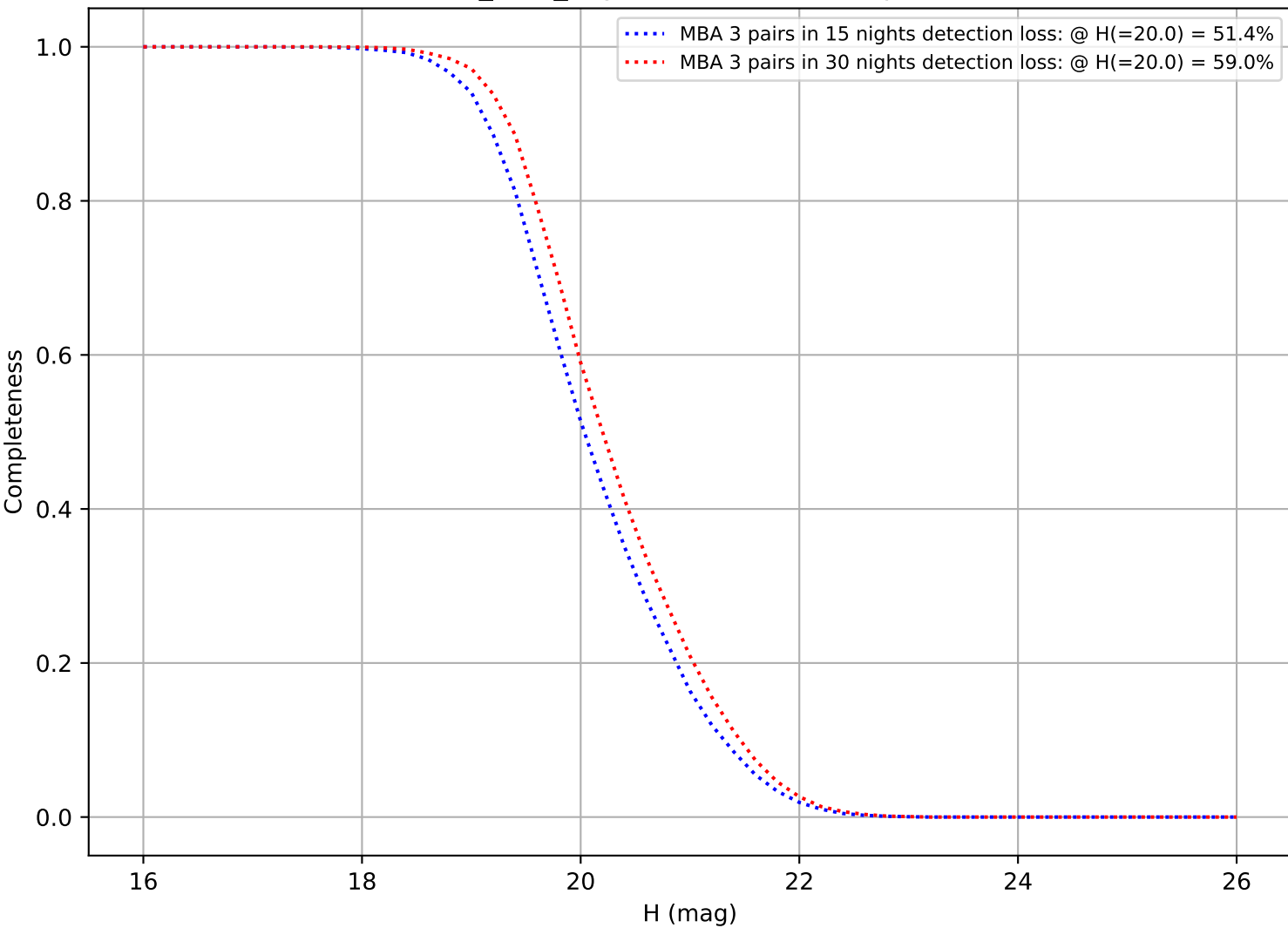
baseline_v3.0_10yrs: DifferentialCompleteness
