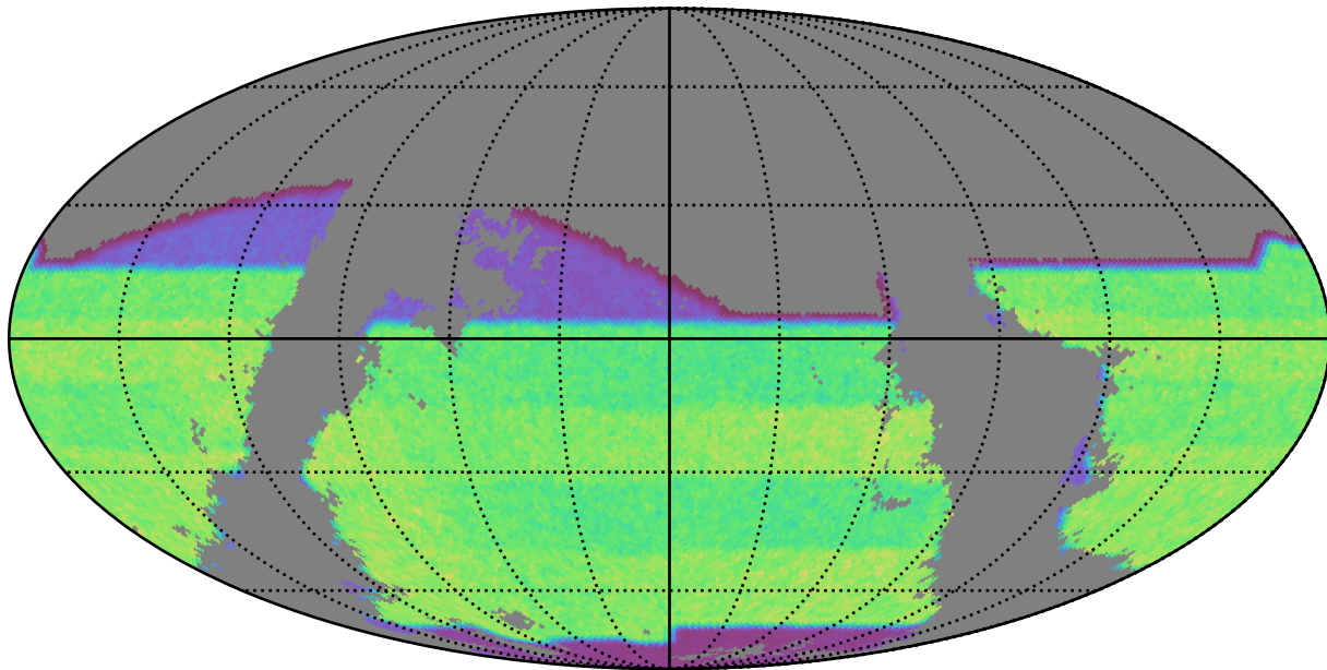
baseline_v3.0_10yrs gri band non-DD: riz_exposure_time_year6
