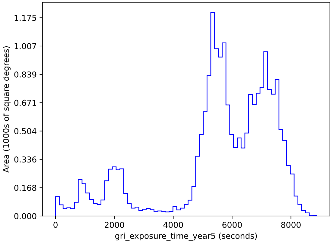
baseline_v3.0_10yrs gri band non-DD: gri_exposure_time_year5
