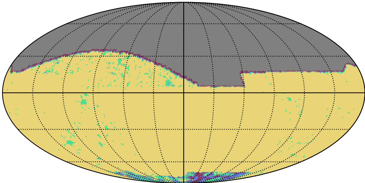
baseline_v3.0_10yrs z band: YearCoverage night
