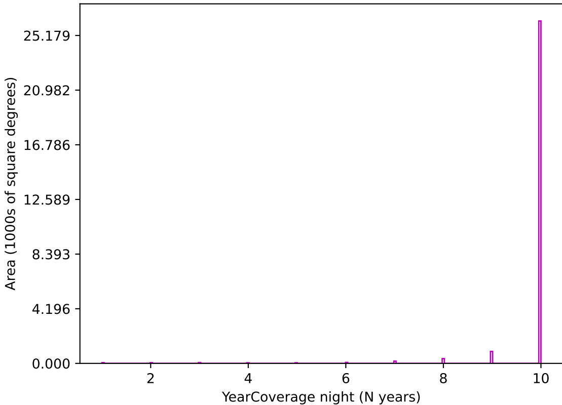
baseline_v3.0_10yrs z band: YearCoverage night
