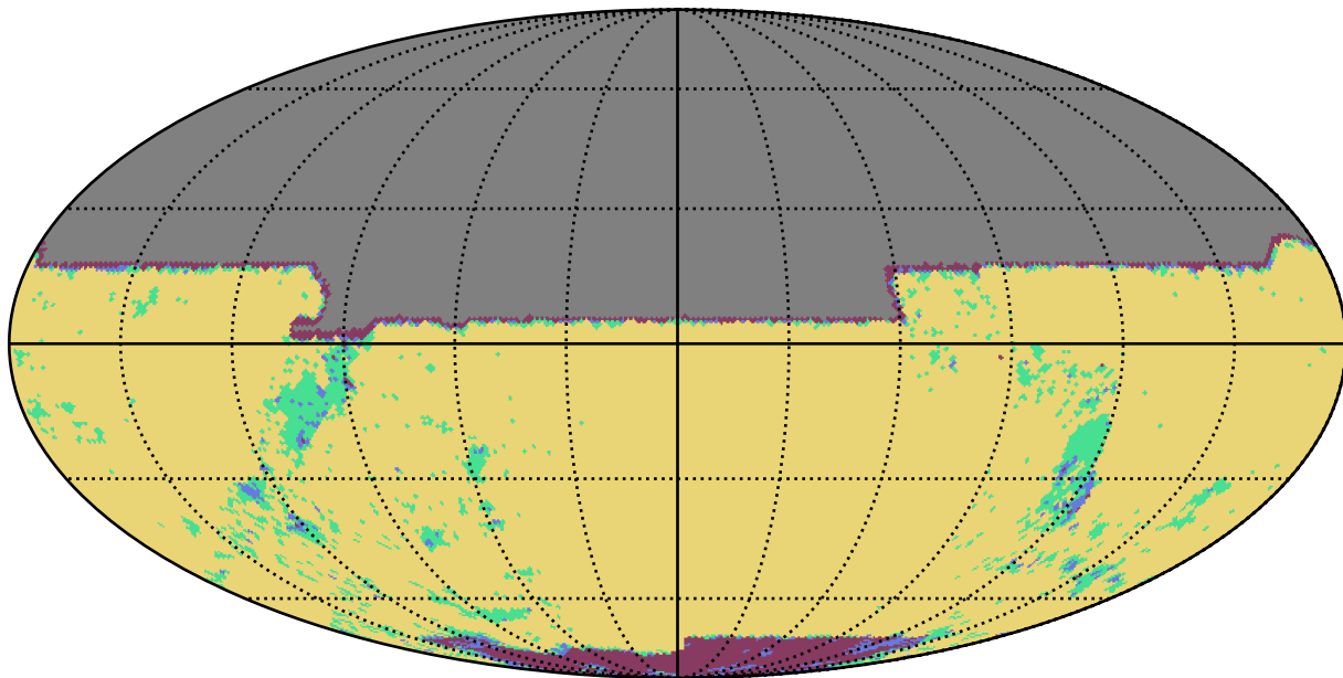
baseline_v3.0_10yrs y band: YearCoverage night
