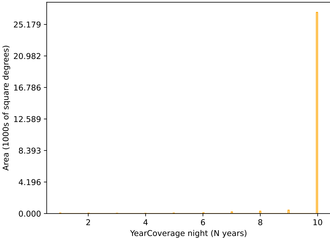
baseline_v3.0_10yrs r band: YearCoverage night
