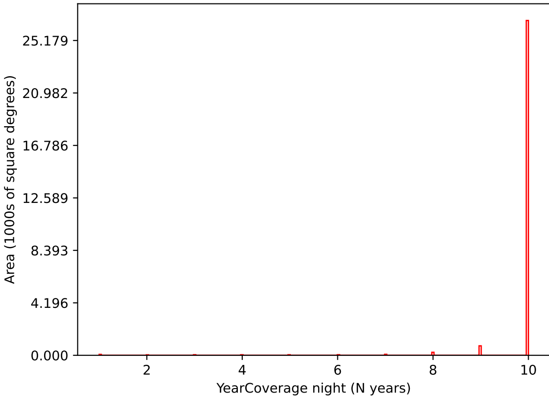
baseline_v3.0_10yrs i band: YearCoverage night
