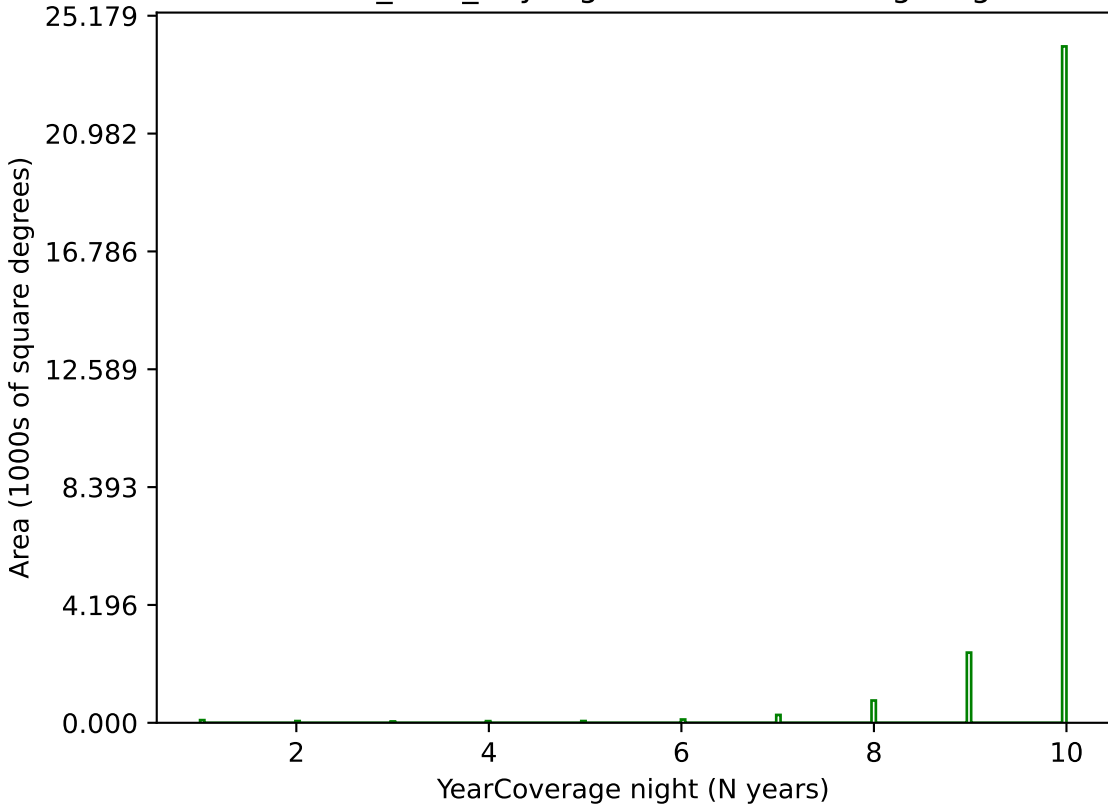
baseline_v3.0_10yrs g band: YearCoverage night
