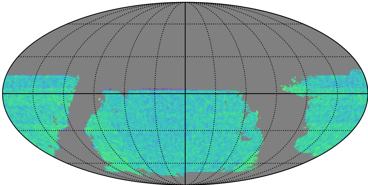
baseline_v3.0_10yrs gri band non-DD: WeakLensingNvisits
