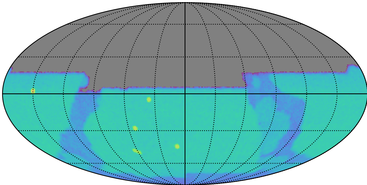
baseline_v3.0_10yrs u: SurfaceBrightLimit
