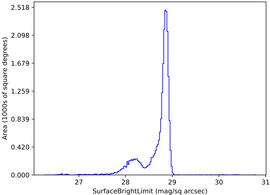
baseline_v3.0_10yrs u: SurfaceBrightLimit
