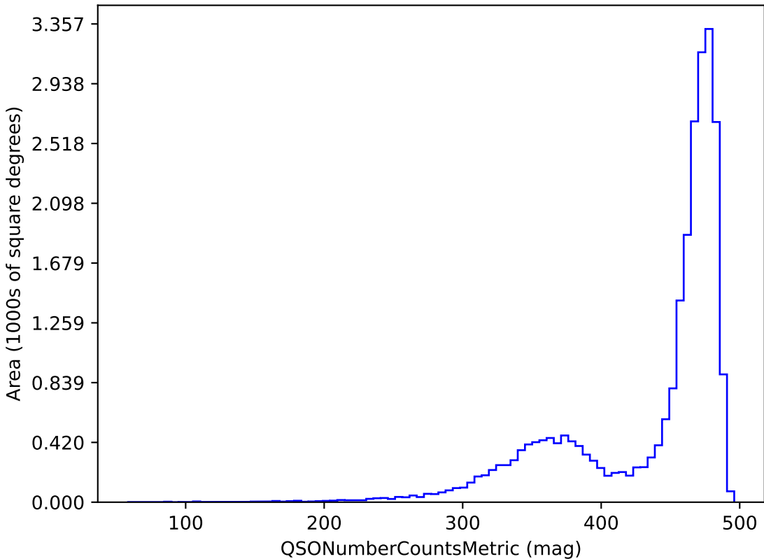
baseline_v3.0_10yrs z band and non-DD: QSONumberCountsMetric
