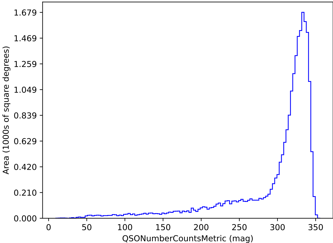
baseline_v3.0_10yrs u band and non-DD: QSONumberCountsMetric
