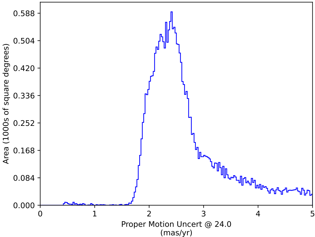
baseline_v3.0_10yrs : Proper Motion Uncert @ 24.0
