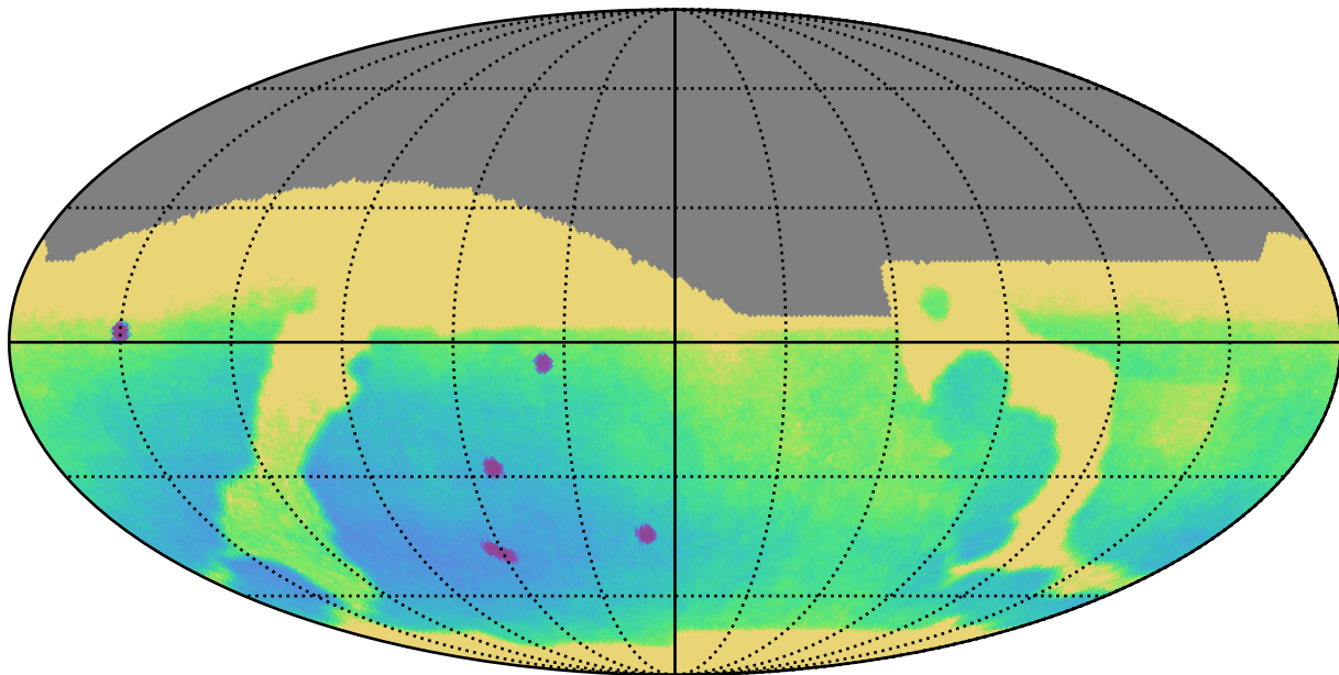
baseline_v3.0_10yrs : Parallax Uncert @ 24.0
