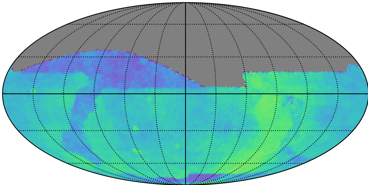
baseline_v3.0_10yrs : Parallax Coverage @ 24.0
