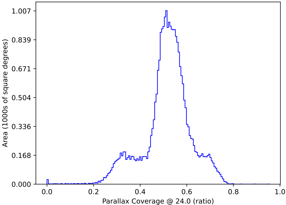
baseline_v3.0_10yrs : Parallax Coverage @ 24.0
