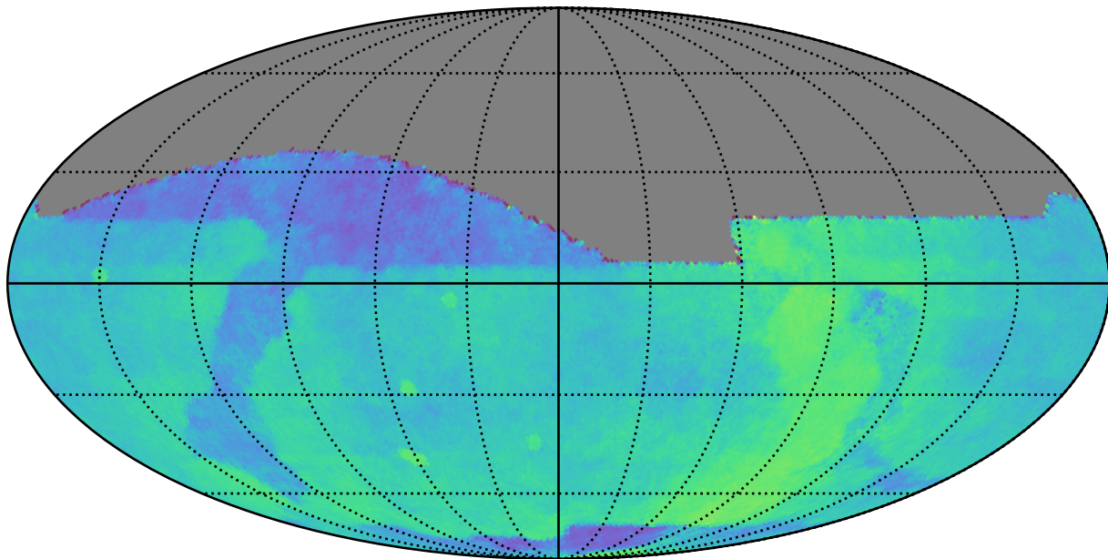
baseline_v3.0_10yrs : Parallax Coverage @ 22.4
