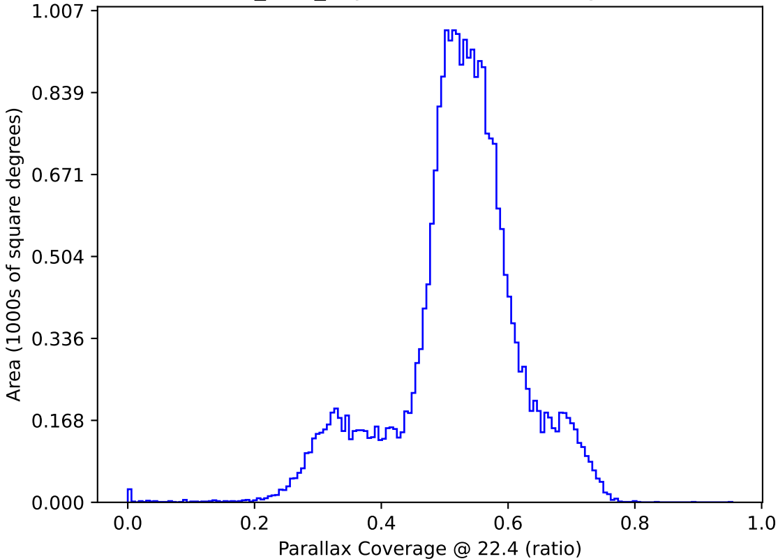
baseline_v3.0_10yrs : Parallax Coverage @ 22.4
