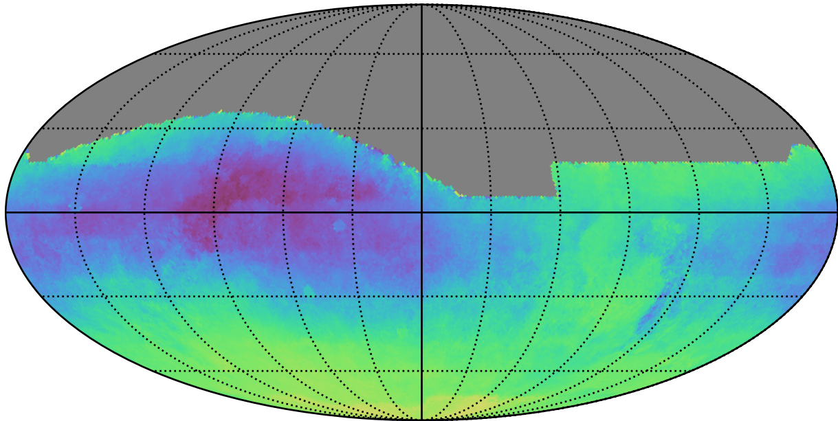
baseline_v3.0_10yrs : Parallax-DCR degeneracy @ 24.0
