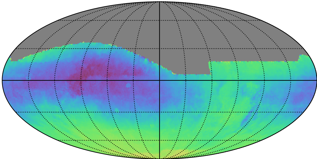
baseline_v3.0_10yrs : Parallax-DCR degeneracy @ 22.4
