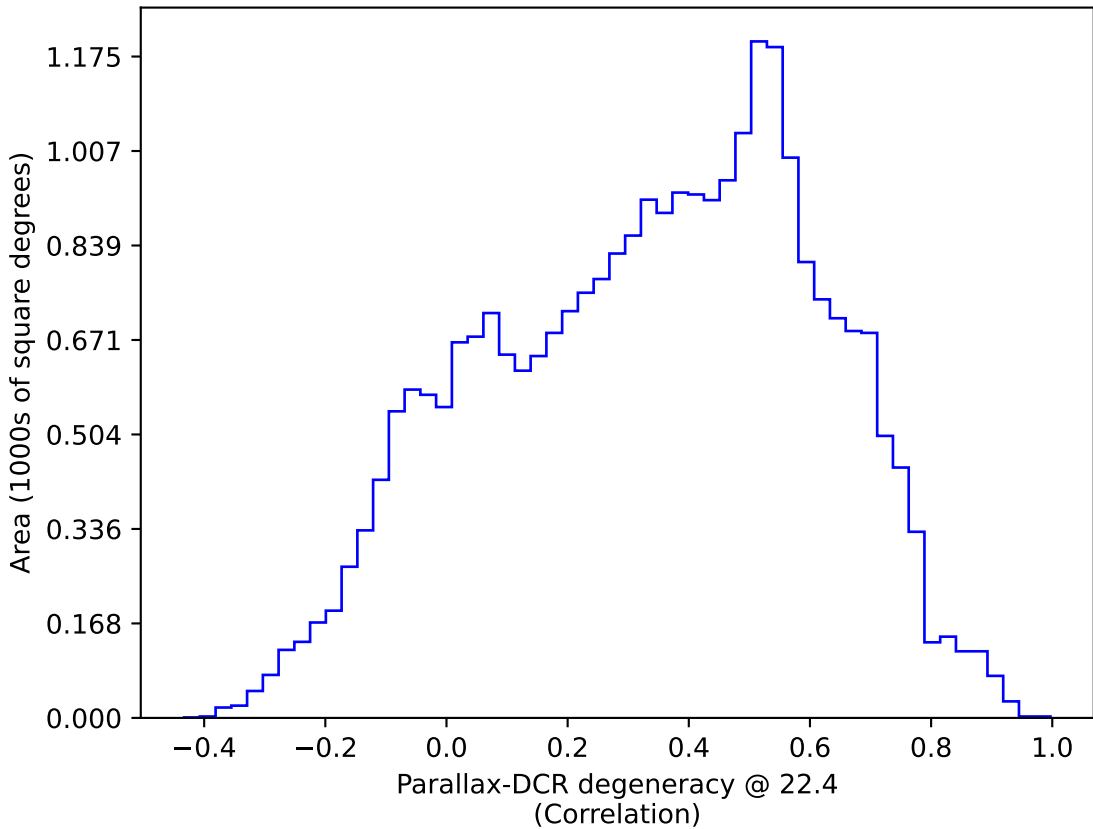
baseline_v3.0_10yrs : Parallax-DCR degeneracy @ 22.4
