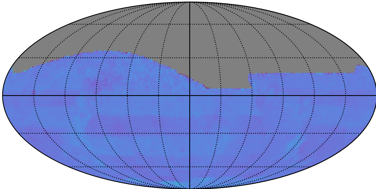
baseline_v3.0_10yrs : Normalized Proper Motion Uncert @ 24.0
