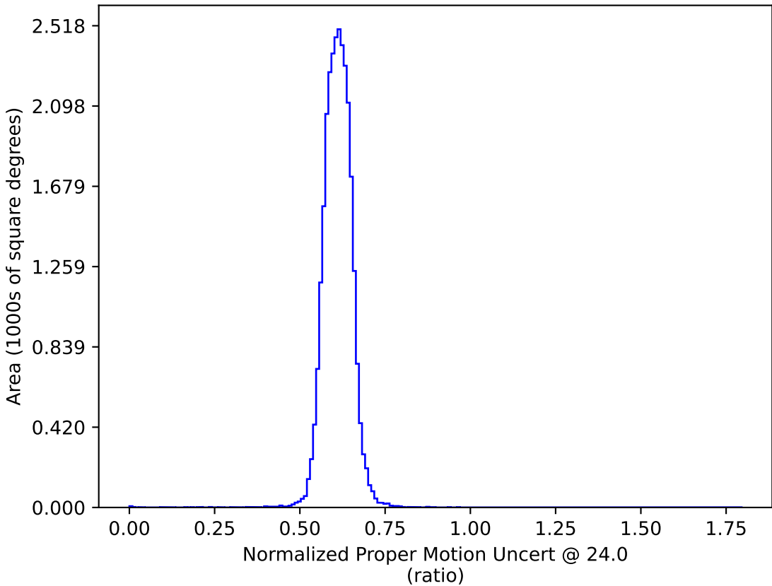
baseline_v3.0_10yrs : Normalized Proper Motion Uncert @ 24.0
