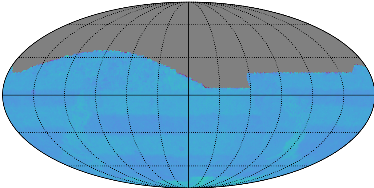
baseline_v3.0_10yrs : Normalized Proper Motion Uncert @ 20.5
