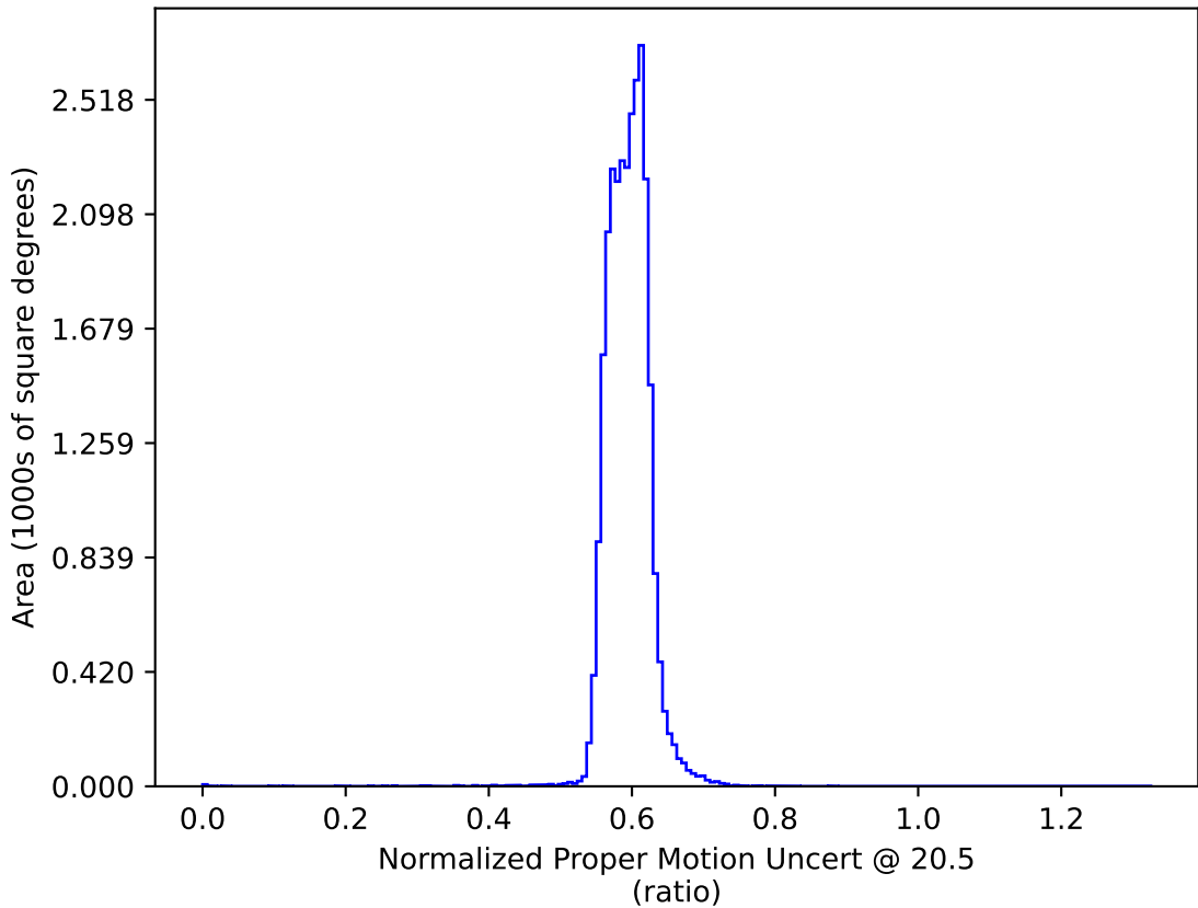
baseline_v3.0_10yrs : Normalized Proper Motion Uncert @ 20.5
