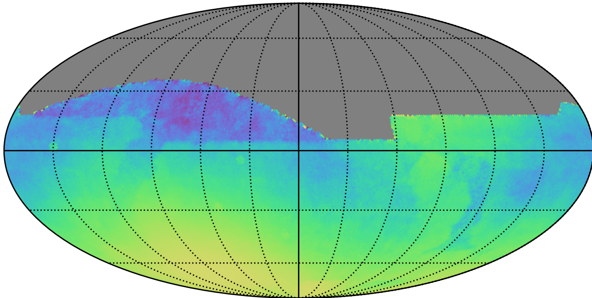
baseline_v3.0_10yrs : Normalized Parallax Uncert @ 24.0
