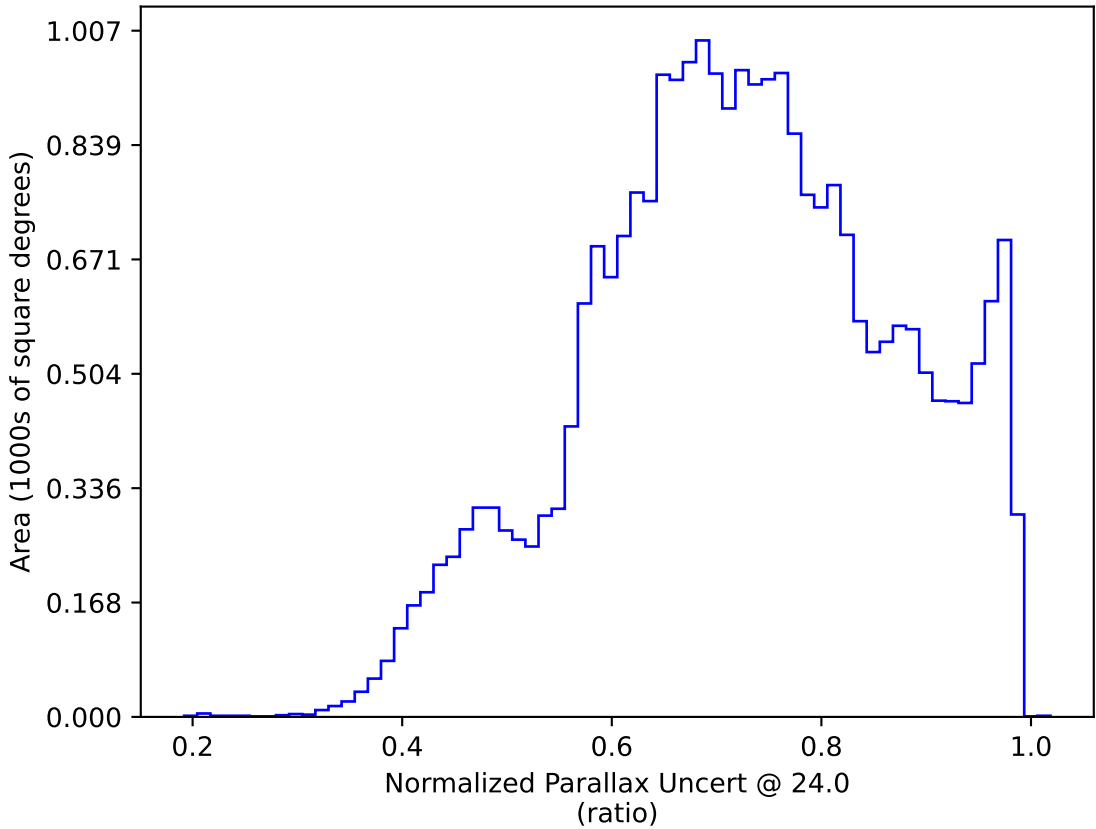
baseline_v3.0_10yrs : Normalized Parallax Uncert @ 24.0
